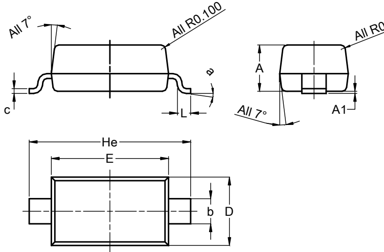
SOD123
